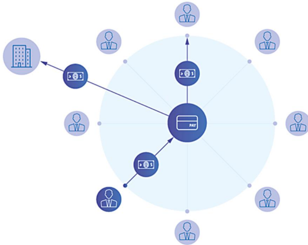
CENTRALIZED SYSTEM
