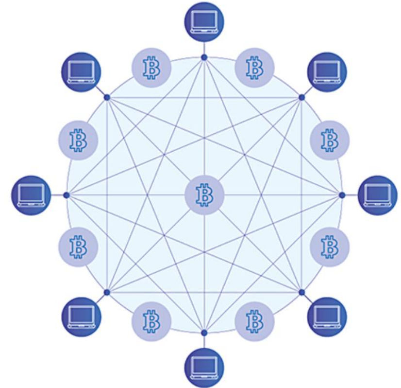
BLOCKCHAIN NETWORK
